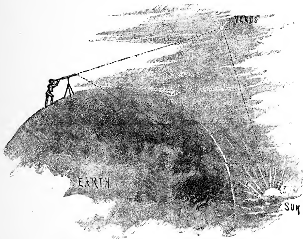
Fig. 49.—To show that Venus shines by Sunlight.
